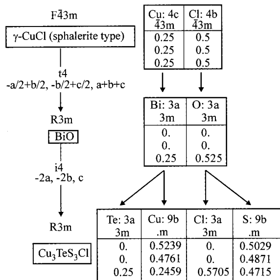
Figure 3. Group–subgroup relationship between \text{CuClCu}_2\text{TeS}_3 and the sphalerite type structure. By means of this “Bärnighausen tree” the symmetry reduction becomes evident in an effective way.
