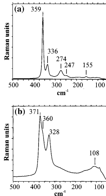
Figure 4. Raman spectra of a) \text{CuClCu}_2\text{TeS}_3 and of b) (\text{CuI})_3\text{Cu}_2\text{TeS}_3 . Both spectra show \nu(\text{Te}-\text{S}) stretching modes for the [\text{TeS}_3]^{2-} group at about 350 \text{cm}^{-1} .
