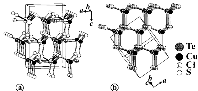
Figure 1. Crystal structures of (a) CuClCu 2 TeS 3 and of (b) \gamma -CuCl (sphalerite type) to show the close structural relationship and also the deviations caused by the 3:1 ordering of both cations and anions.
